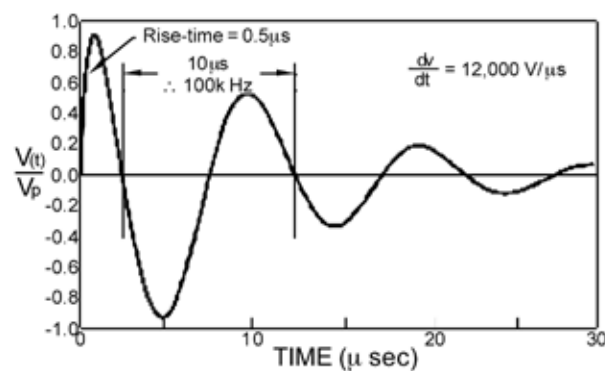
100 kHz Ring Wave (Figure 2)
